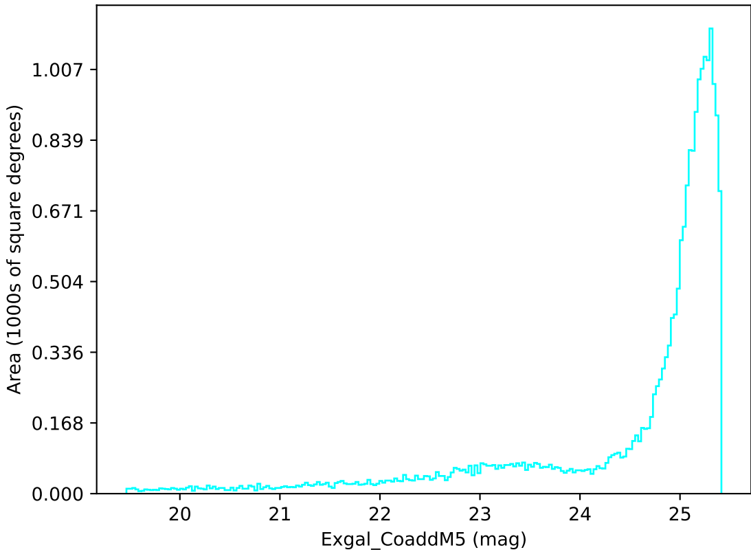
weather_cloudso6v3.4_10yrs All sky u band: Exgal_CoaddM5
