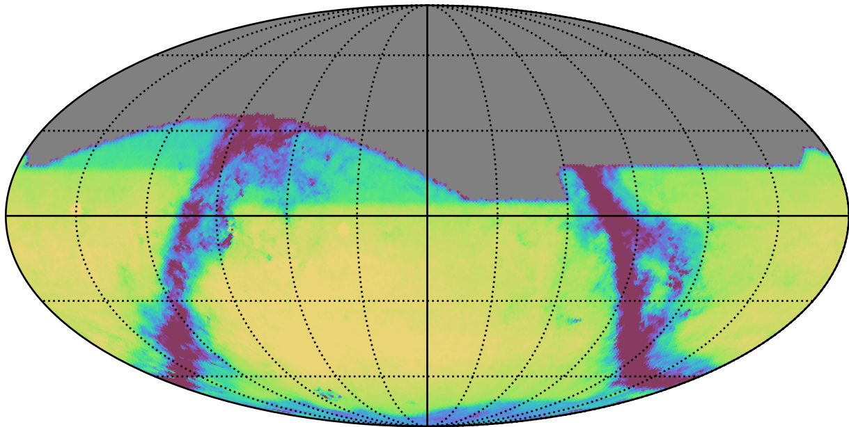
weather_cloudso6v3.4_10yrs All sky r band: Exgal_CoaddM5
