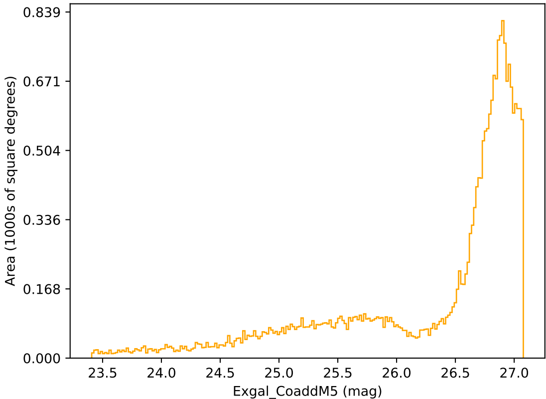
weather_cloudso6v3.4_10yrs All sky r band: Exgal_CoaddM5
