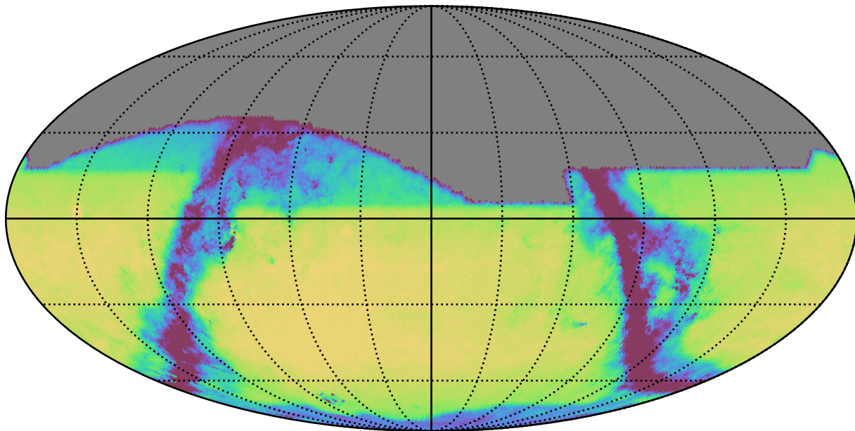
weather_cloudso6v3.4_10yrs All sky i band: Exgal_CoaddM5
