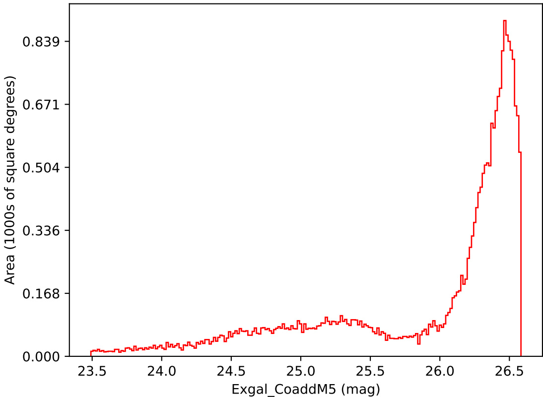
weather_cloudso6v3.4_10yrs All sky i band: Exgal_CoaddM5
