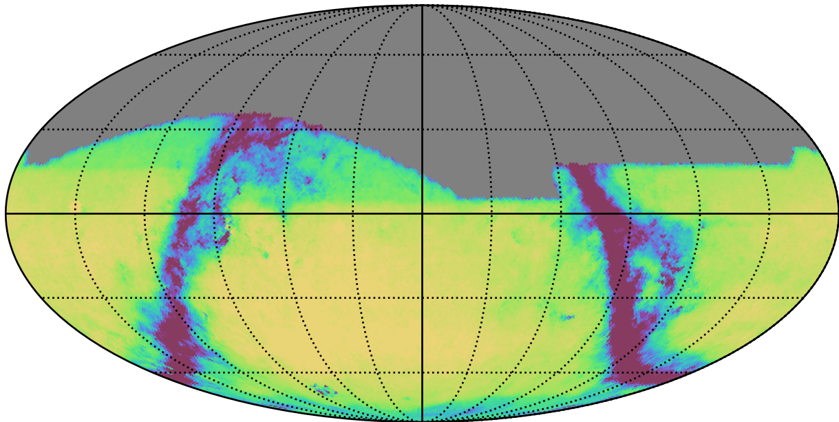
weather_cloudso6v3.4_10yrs All sky g band: Exgal_CoaddM5
