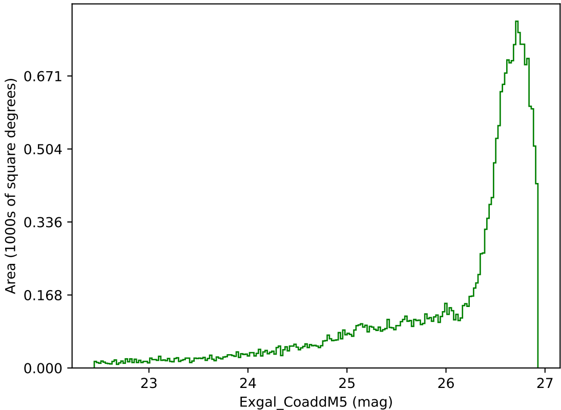
weather_cloudso6v3.4_10yrs All sky g band: Exgal_CoaddM5
