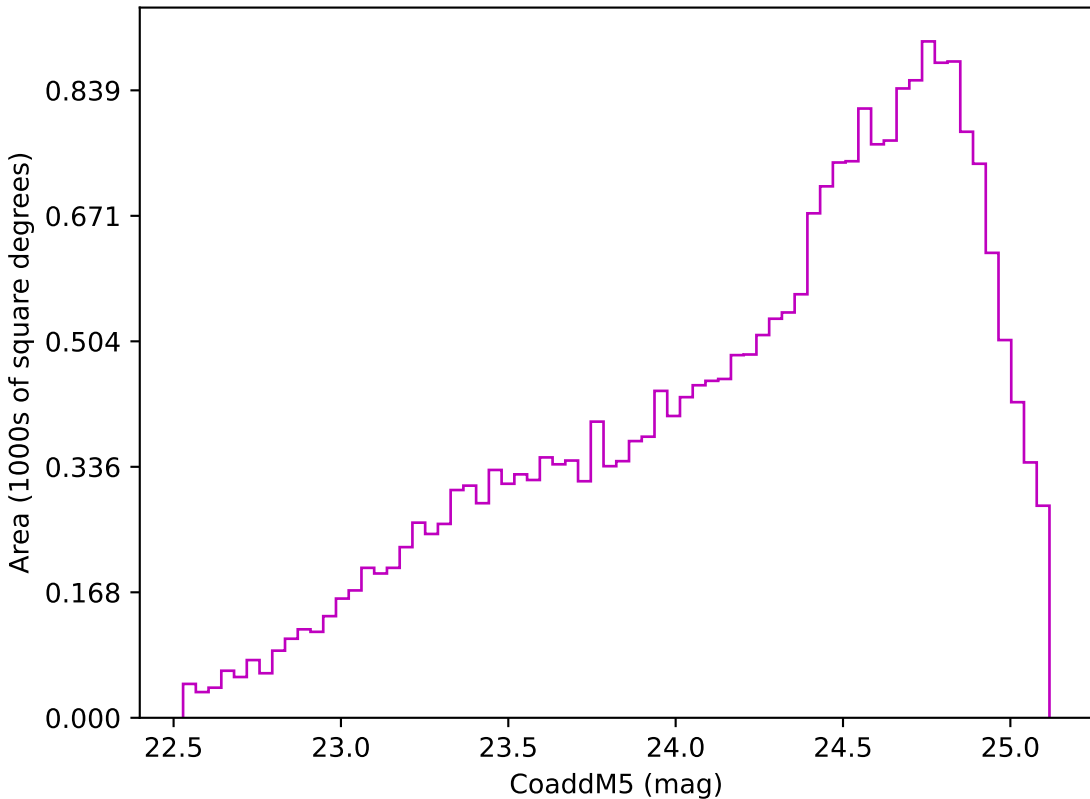
weather_cloudso6v3.4_10yrs Yr 3-4 z band: CoaddM5
