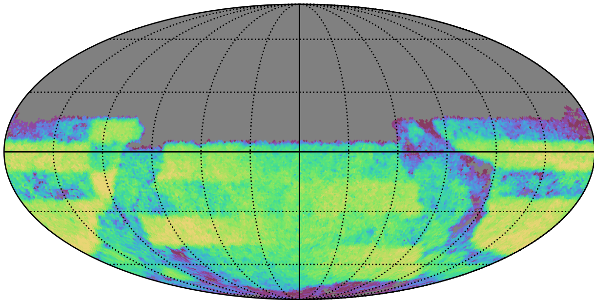
weather_cloudso6v3.4_10yrs Yr 3-4 y band: CoaddM5
