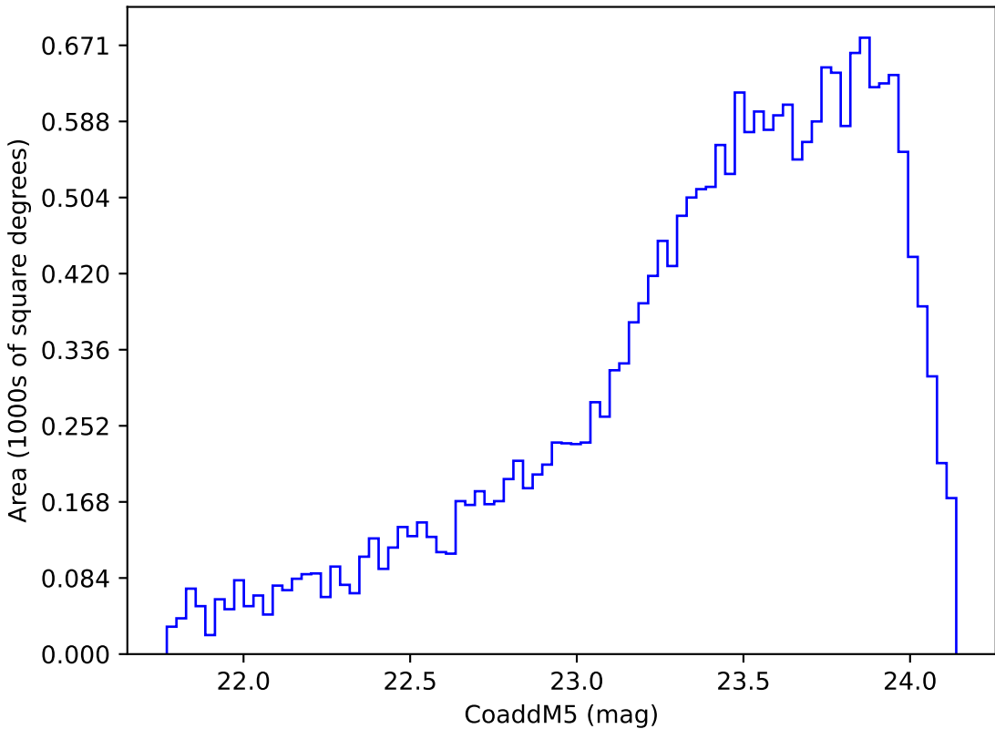
weather_cloudso6v3.4_10yrs Yr 3-4 y band: CoaddM5
