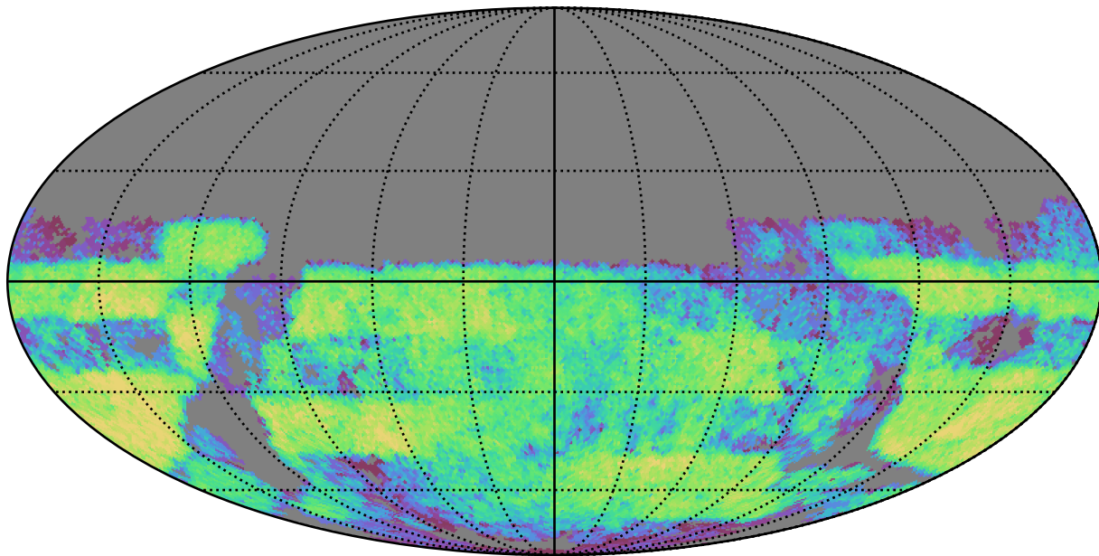
weather_cloudso6v3.4_10yrs Yr 3-4 u band: CoaddM5
