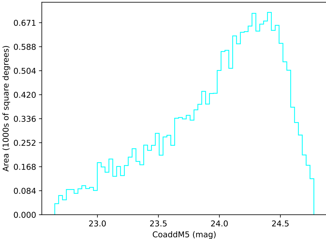
weather_cloudso6v3.4_10yrs Yr 3-4 u band: CoaddM5
