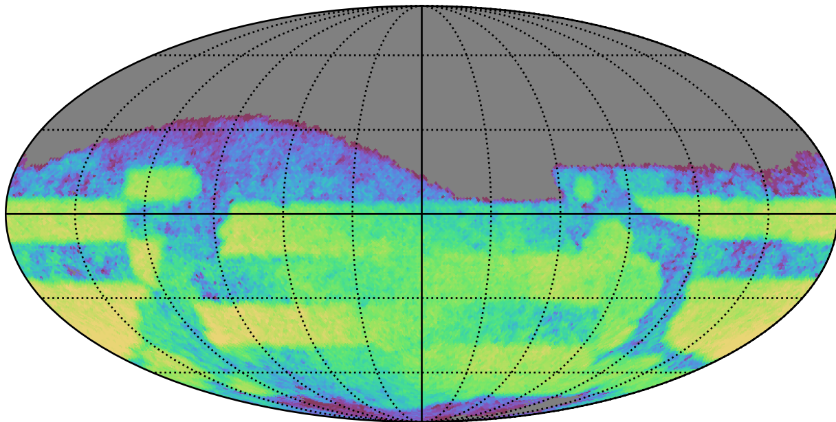
weather_cloudso6v3.4_10yrs Yr 3-4 r band: CoaddM5
