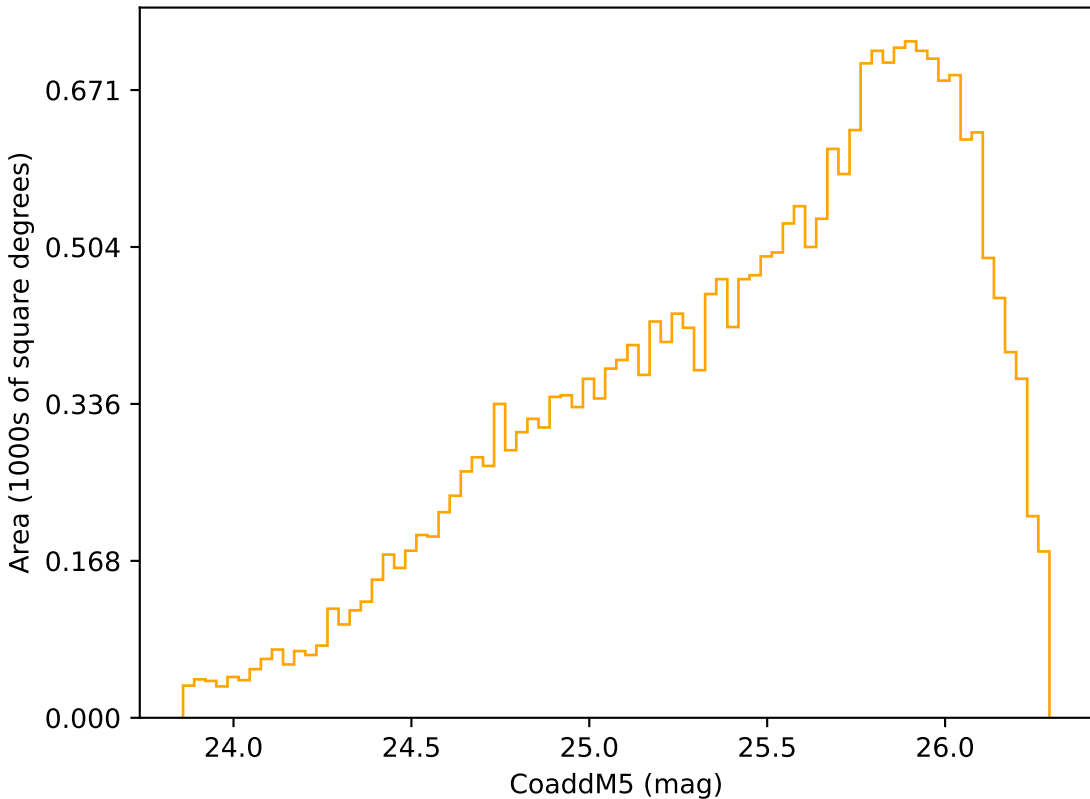
weather_cloudso6v3.4_10yrs Yr 3-4 r band: CoaddM5
