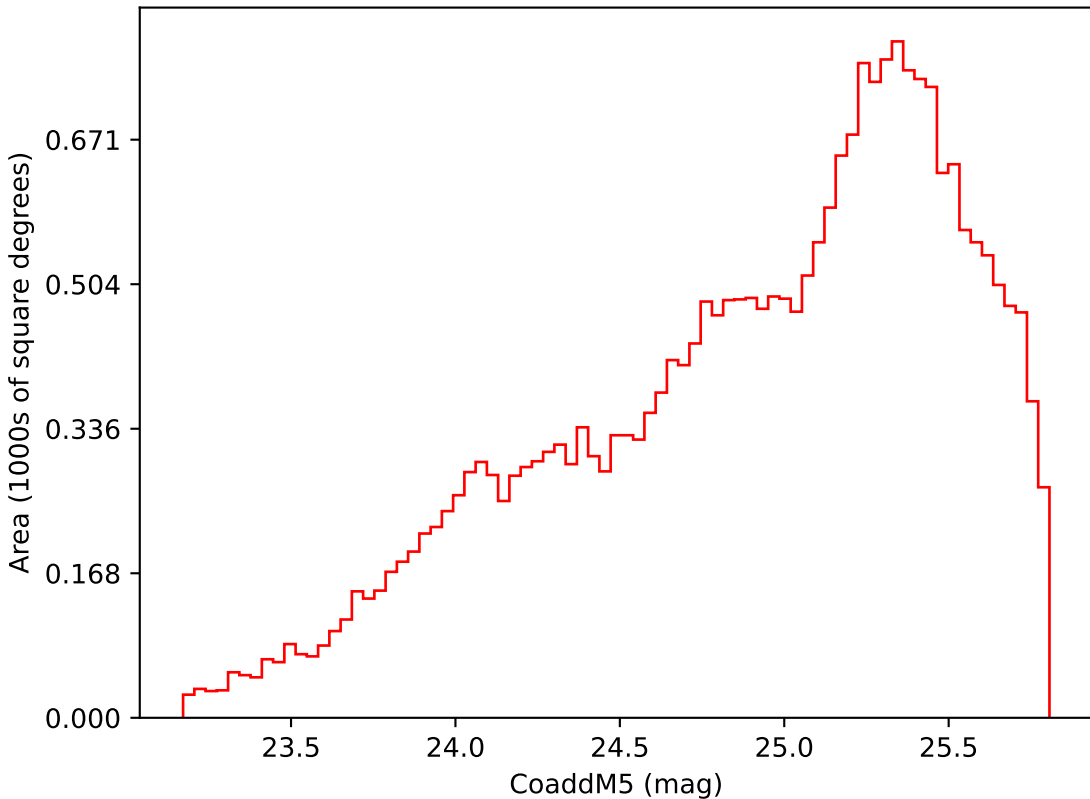
weather_cloudso6v3.4_10yrs Yr 3-4 i band: CoaddM5
