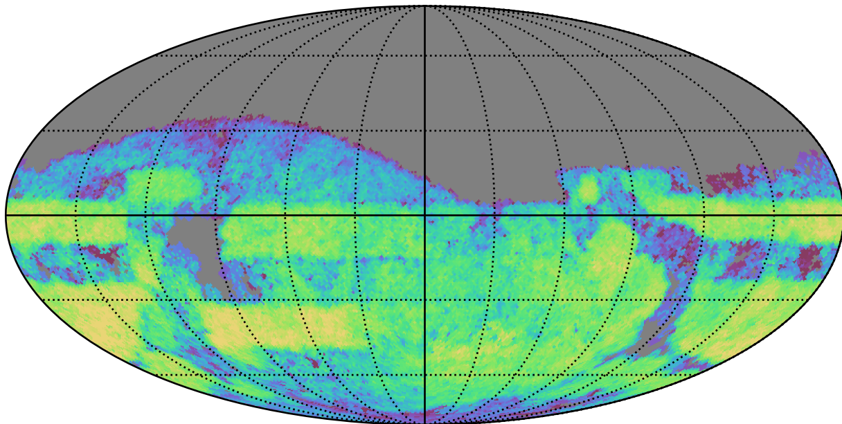
weather_cloudso6v3.4_10yrs Yr 3-4 g band: CoaddM5
