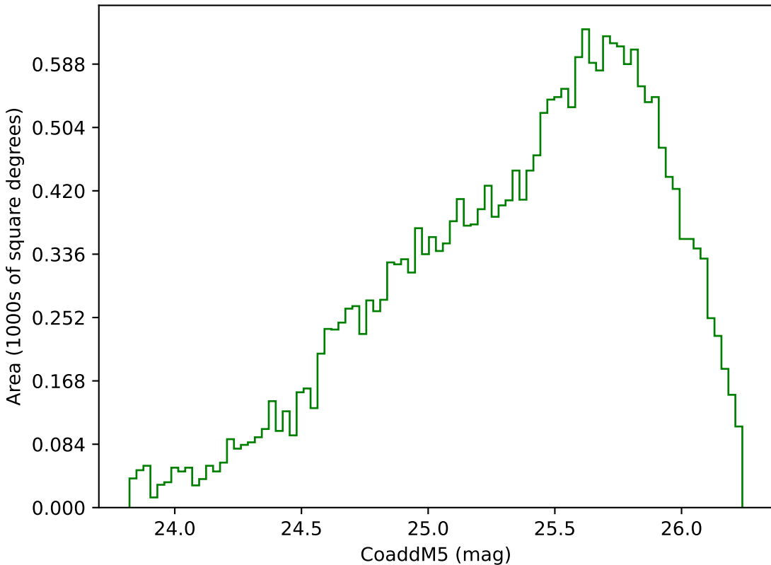
weather_cloudso6v3.4_10yrs Yr 3-4 g band: CoaddM5
