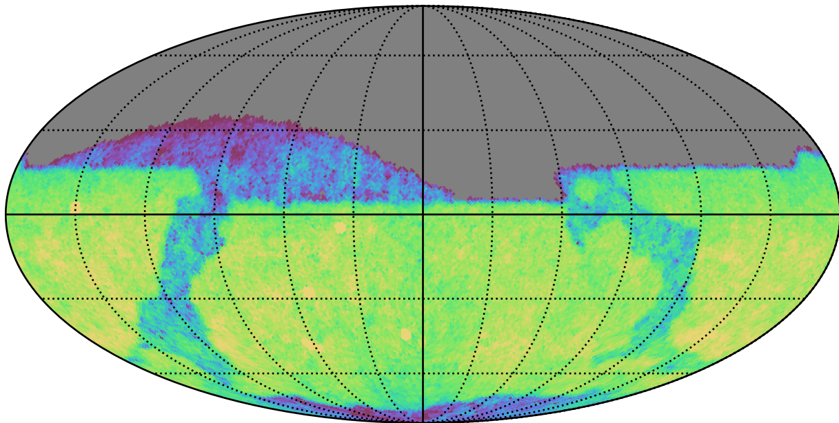
weather_cloudso6v3.4_10yrs Yr 1 z band: CoaddM5
