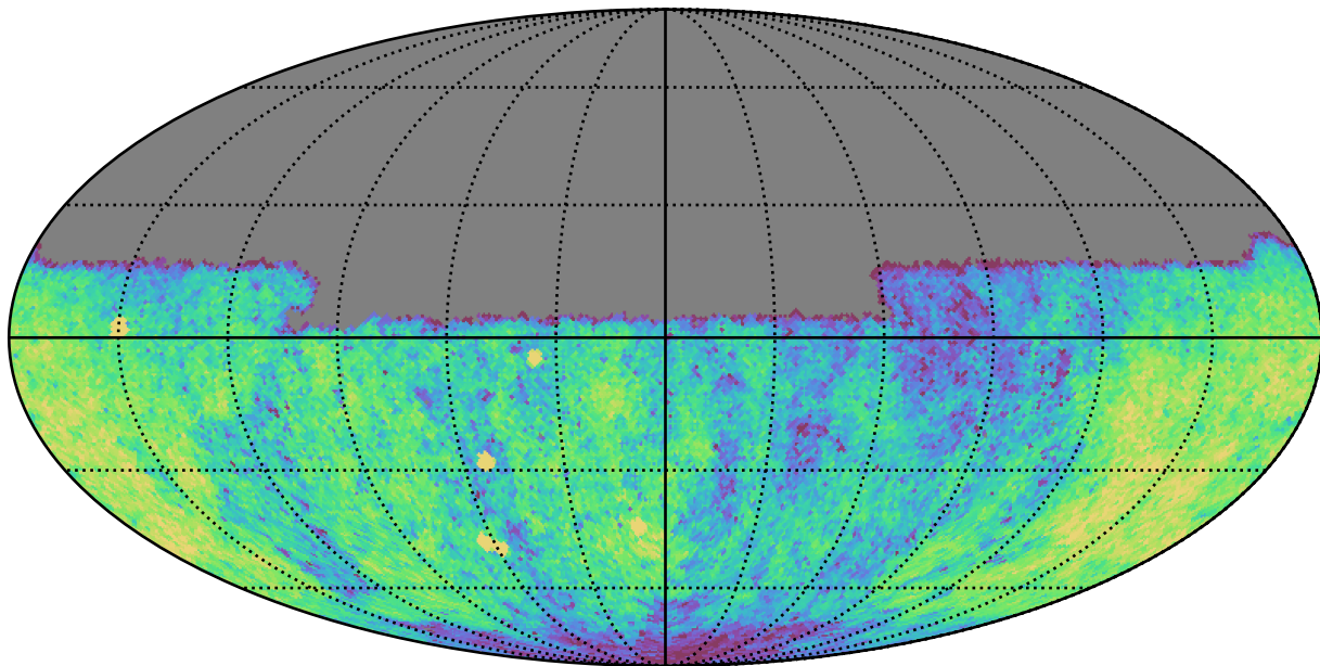
weather_cloudso6v3.4_10yrs Yr 1 u band: CoaddM5
