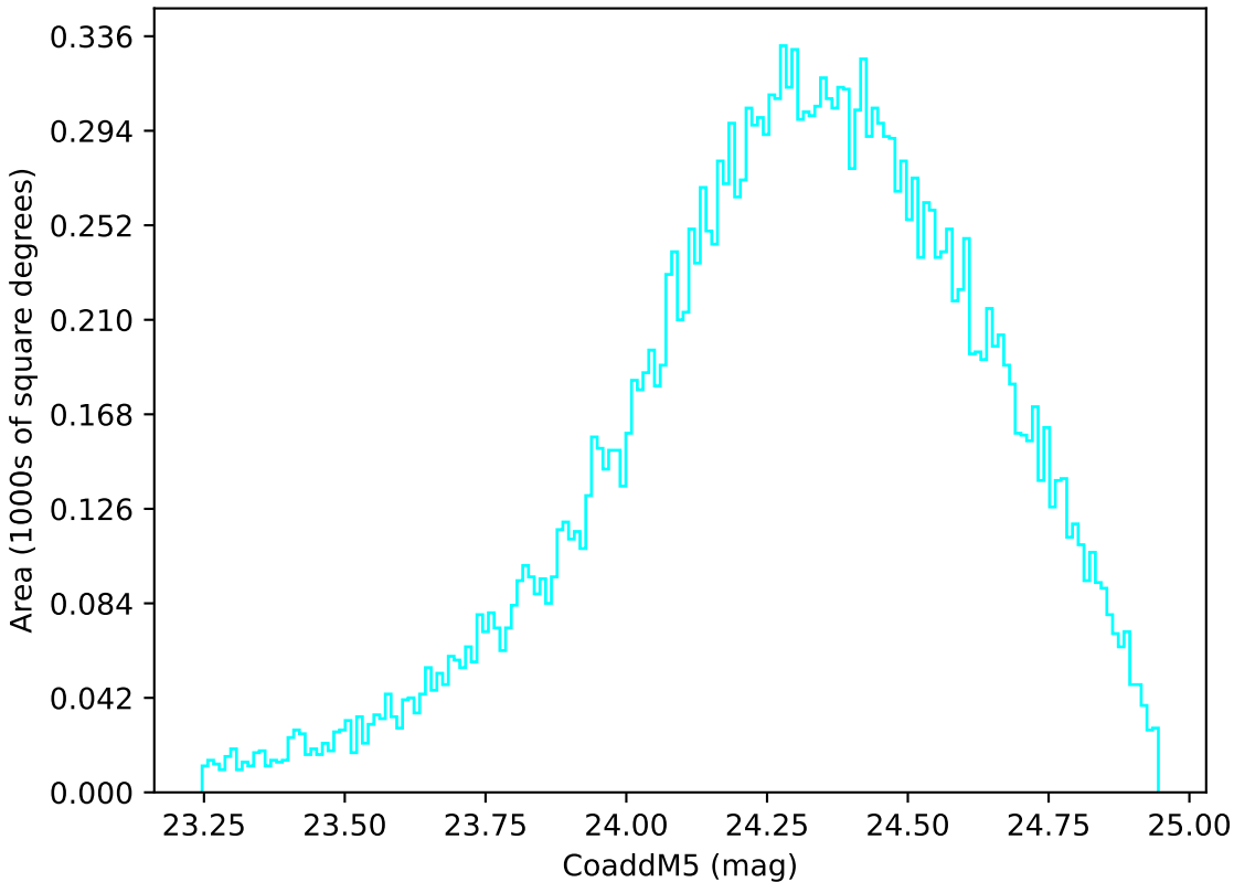
weather_cloudso6v3.4_10yrs Yr 1 u band: CoaddM5
