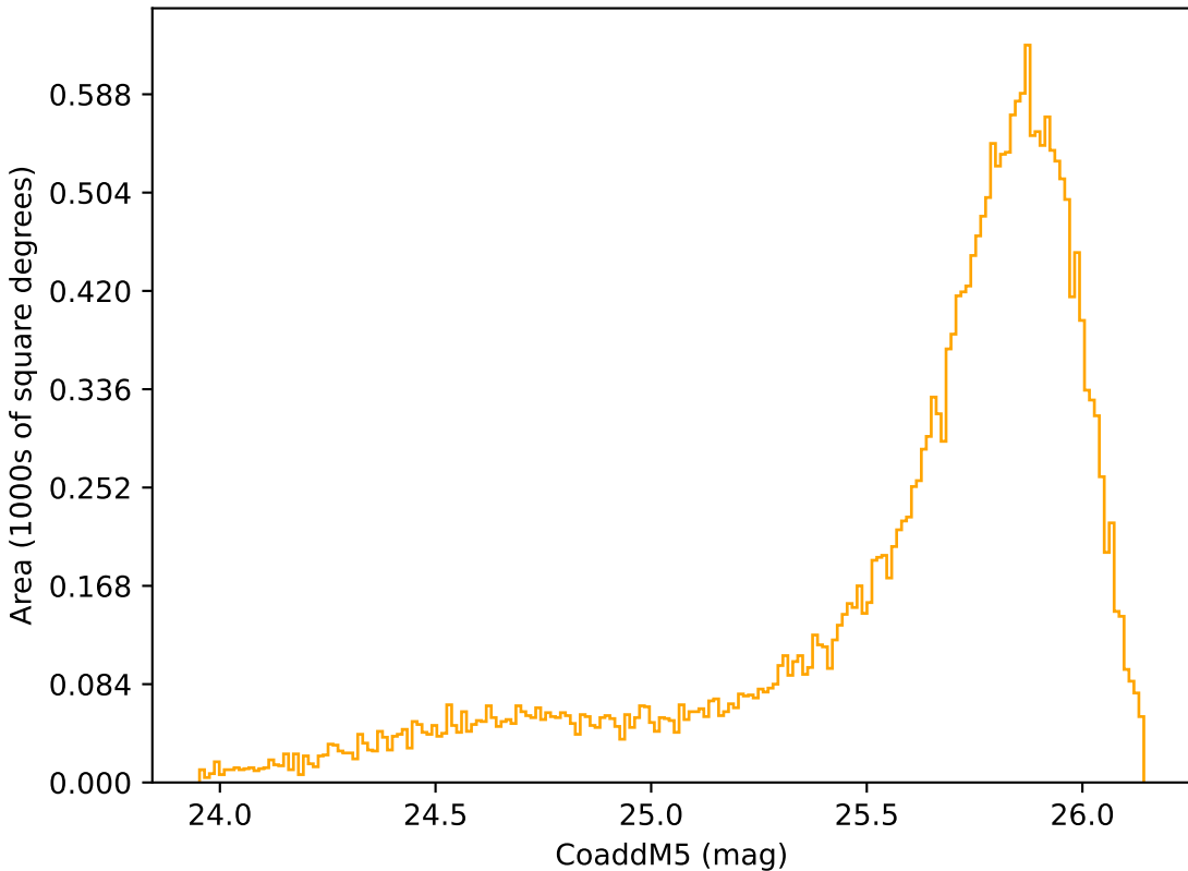
weather_cloudso6v3.4_10yrs Yr 1 r band: CoaddM5
