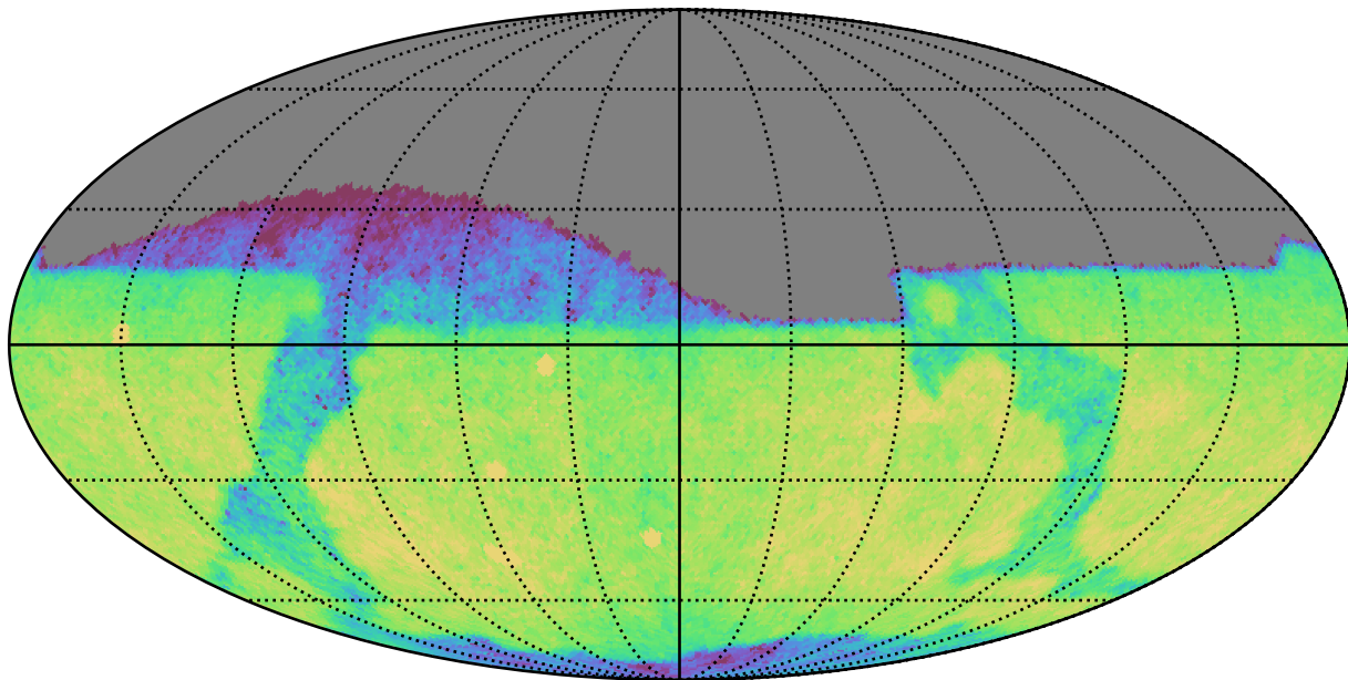
weather_cloudso6v3.4_10yrs Yr 1 i band: CoaddM5
