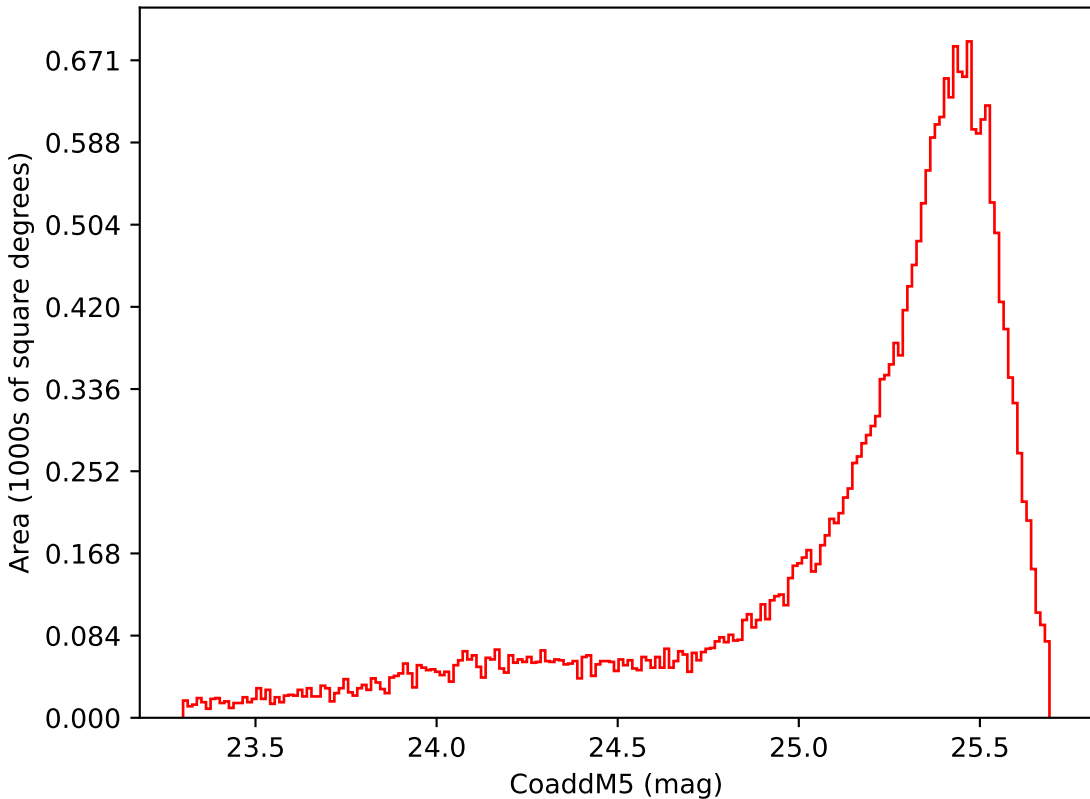
weather_cloudso6v3.4_10yrs Yr 1 i band: CoaddM5
