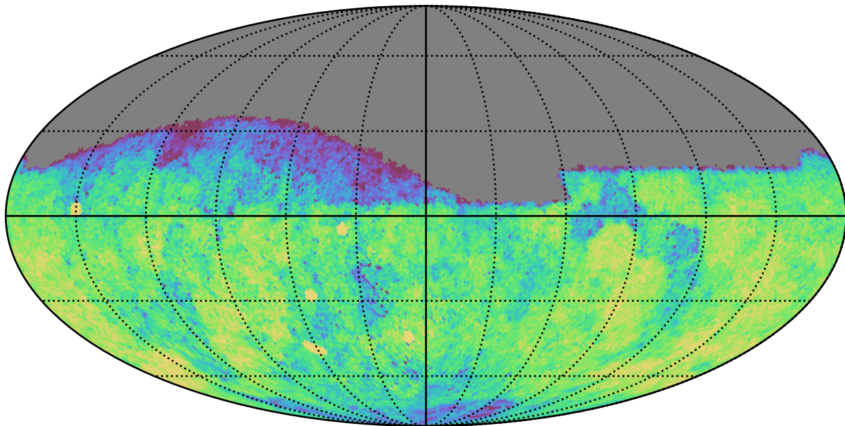
weather_cloudso6v3.4_10yrs Yr 1 g band: CoaddM5
