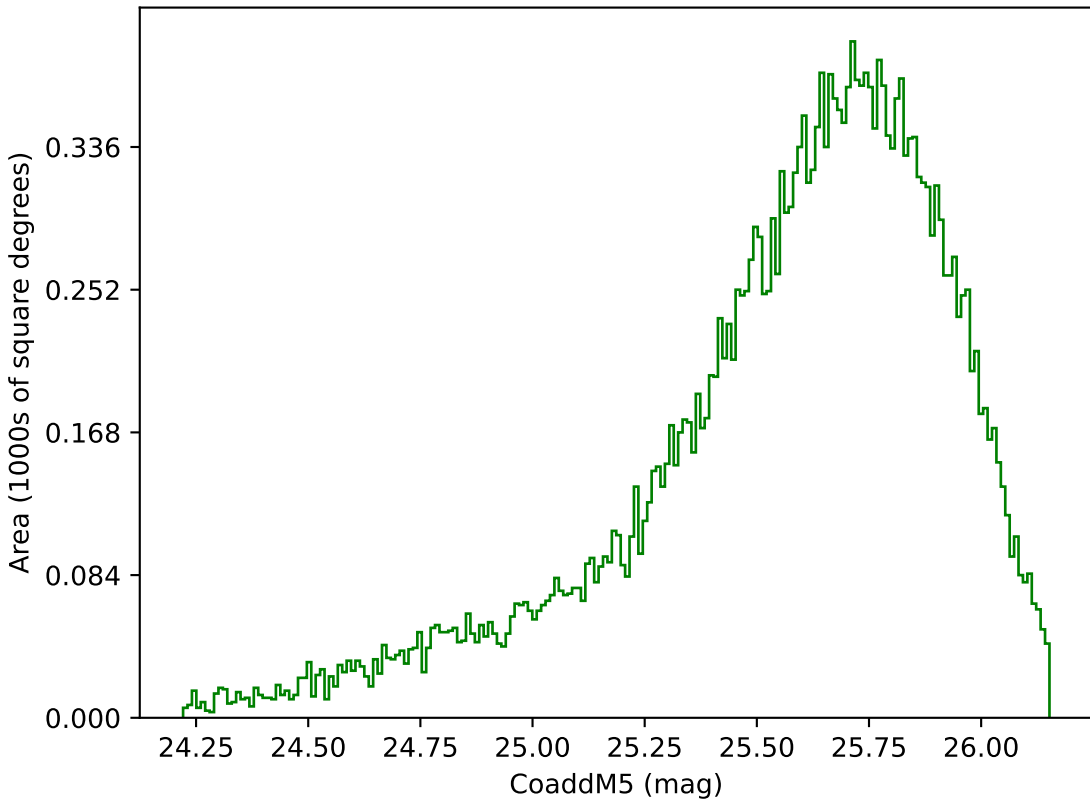
weather_cloudso6v3.4_10yrs Yr 1 g band: CoaddM5
