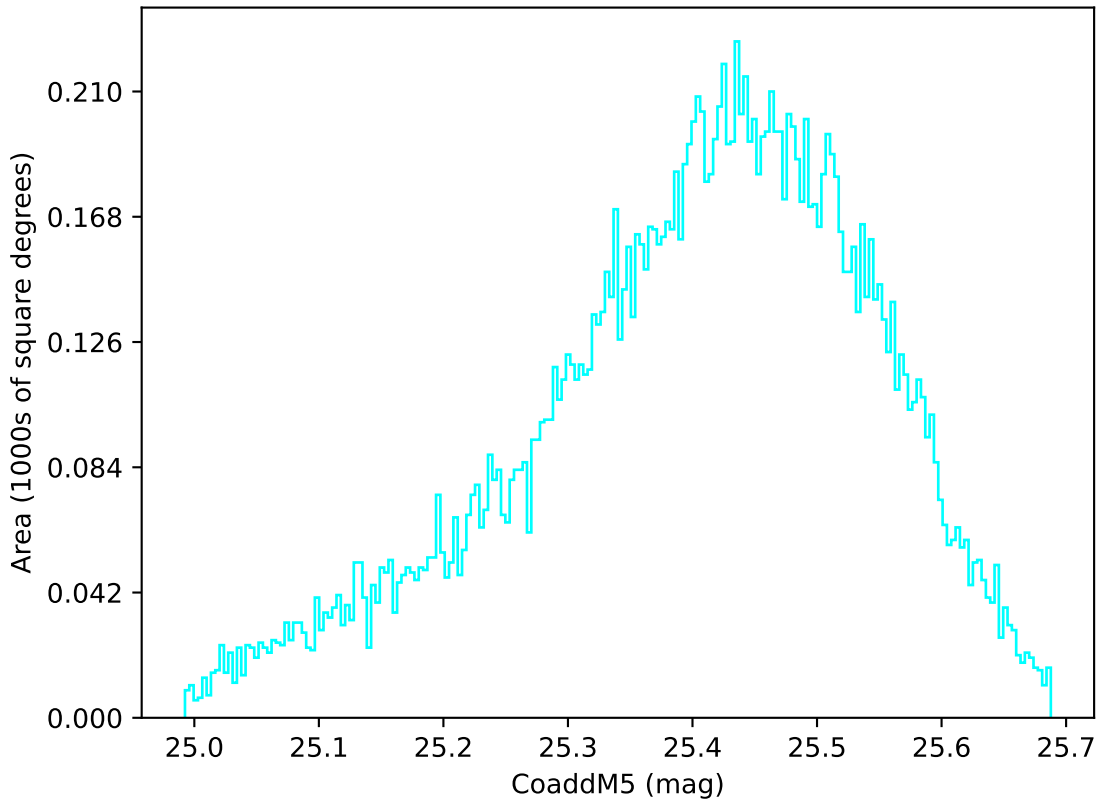
weather_cloudso6v3.4_10yrs WFD u band: CoaddM5
