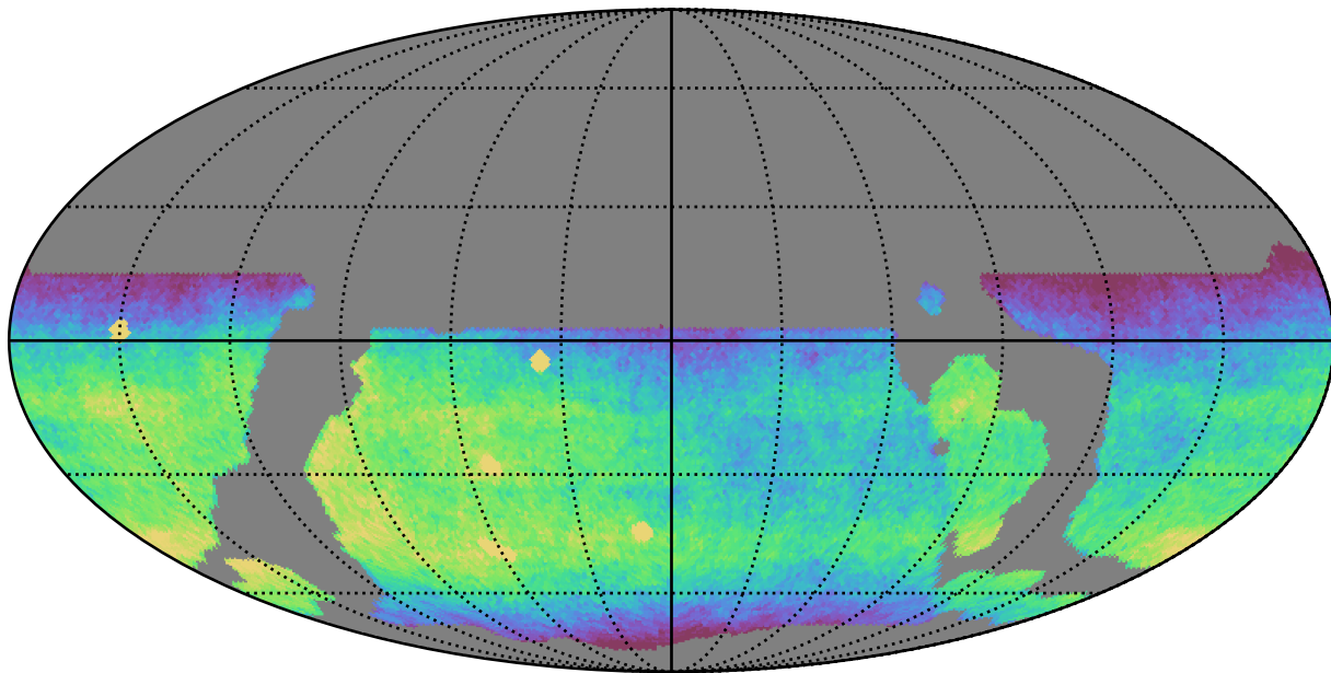
weather_cloudso6v3.4_10yrs WFD r band: CoaddM5
