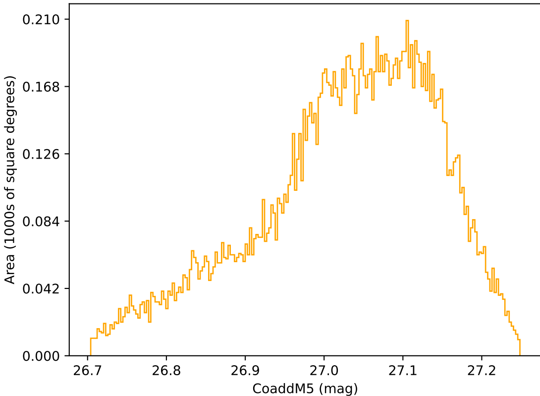
weather_cloudso6v3.4_10yrs WFD r band: CoaddM5
