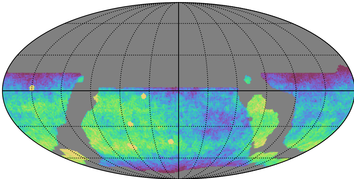
weather_cloudso6v3.4_10yrs WFD g band: CoaddM5
