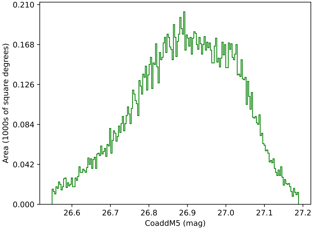
weather_cloudso6v3.4_10yrs WFD g band: CoaddM5
