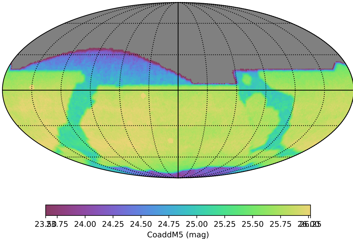
weather_cloudso6v3.4_10yrs All sky z band: CoaddM5
