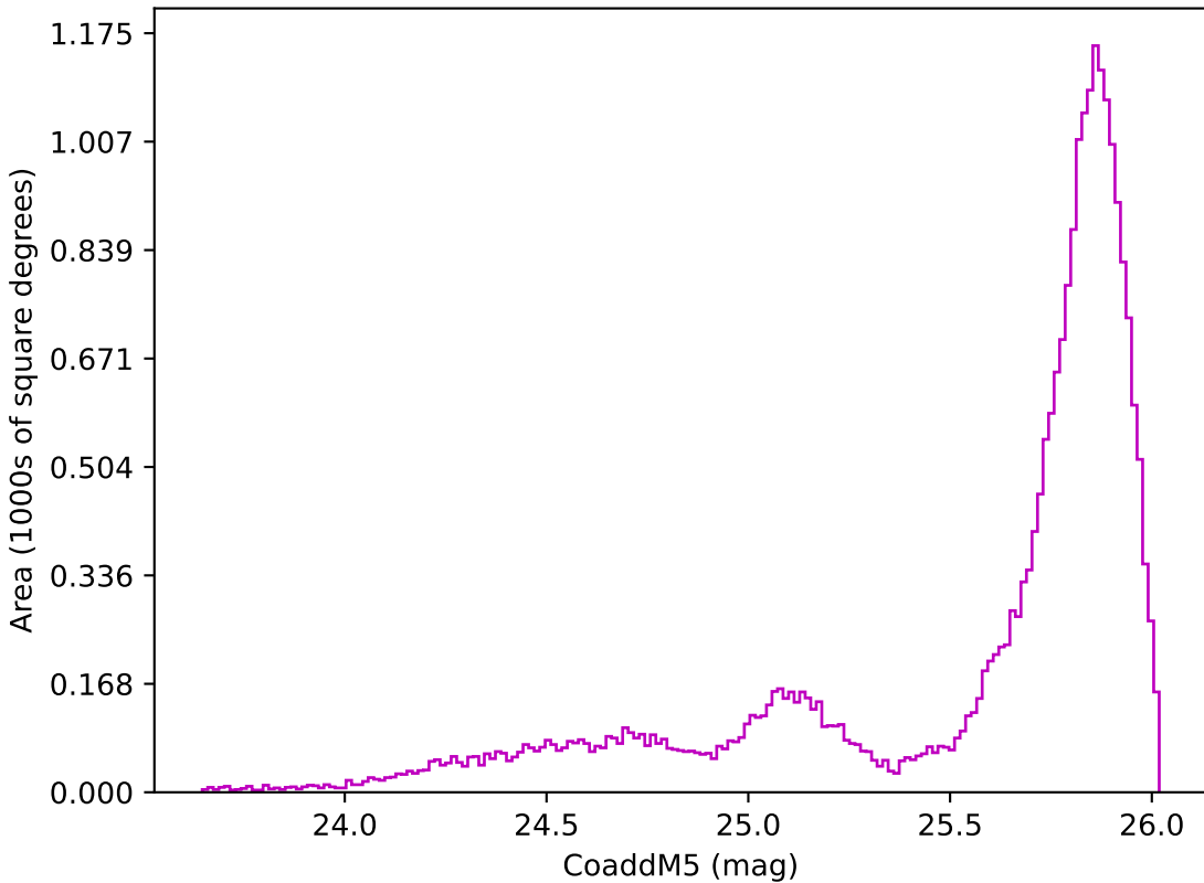
weather_cloudso6v3.4_10yrs All sky z band: CoaddM5
