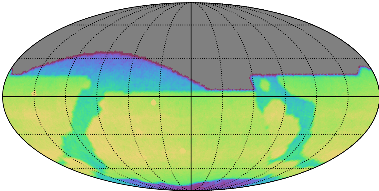
weather_cloudso6v3.4_10yrs All sky r band: CoaddM5
