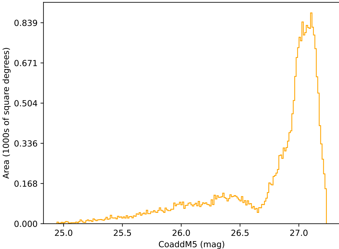
weather_cloudso6v3.4_10yrs All sky r band: CoaddM5
