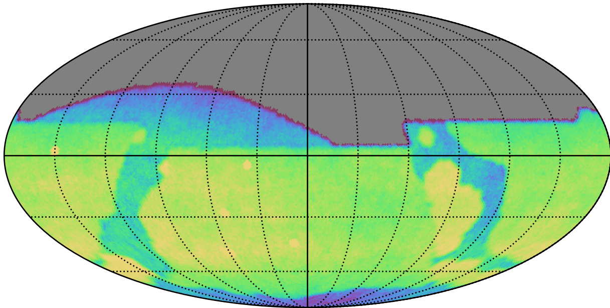
weather_cloudso6v3.4_10yrs All sky g band: CoaddM5
