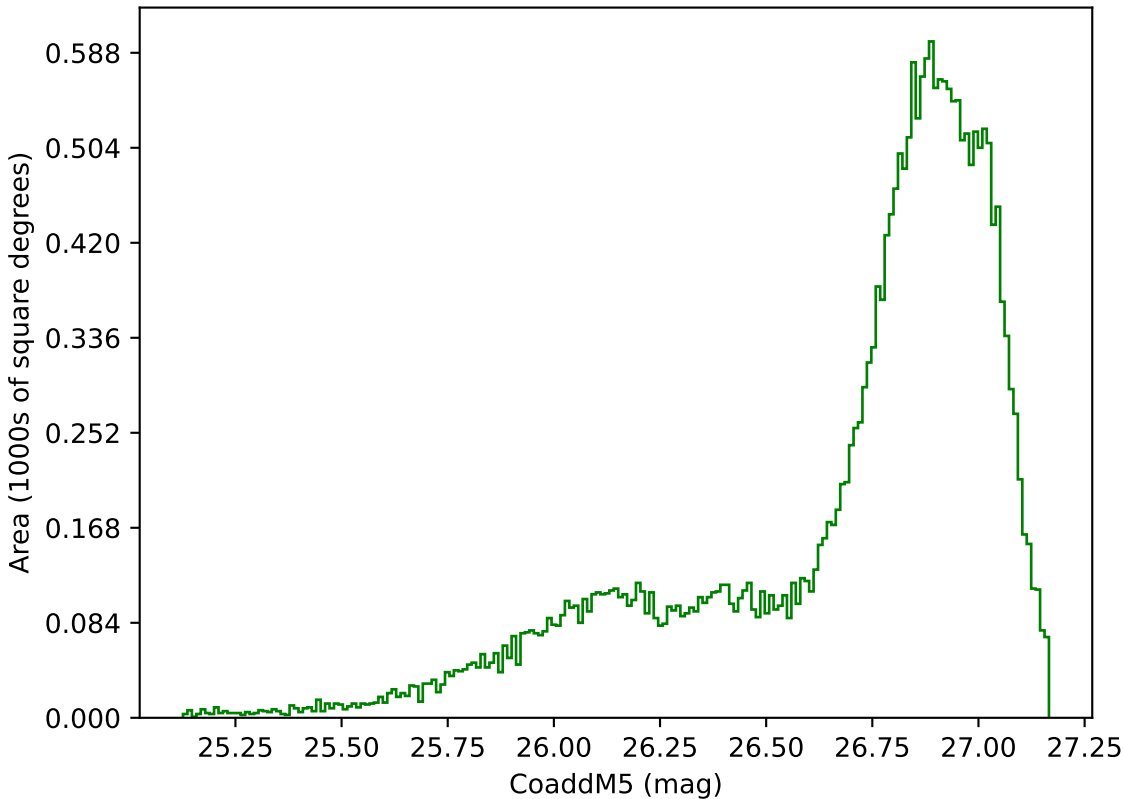
weather_cloudso6v3.4_10yrs All sky g band: CoaddM5
