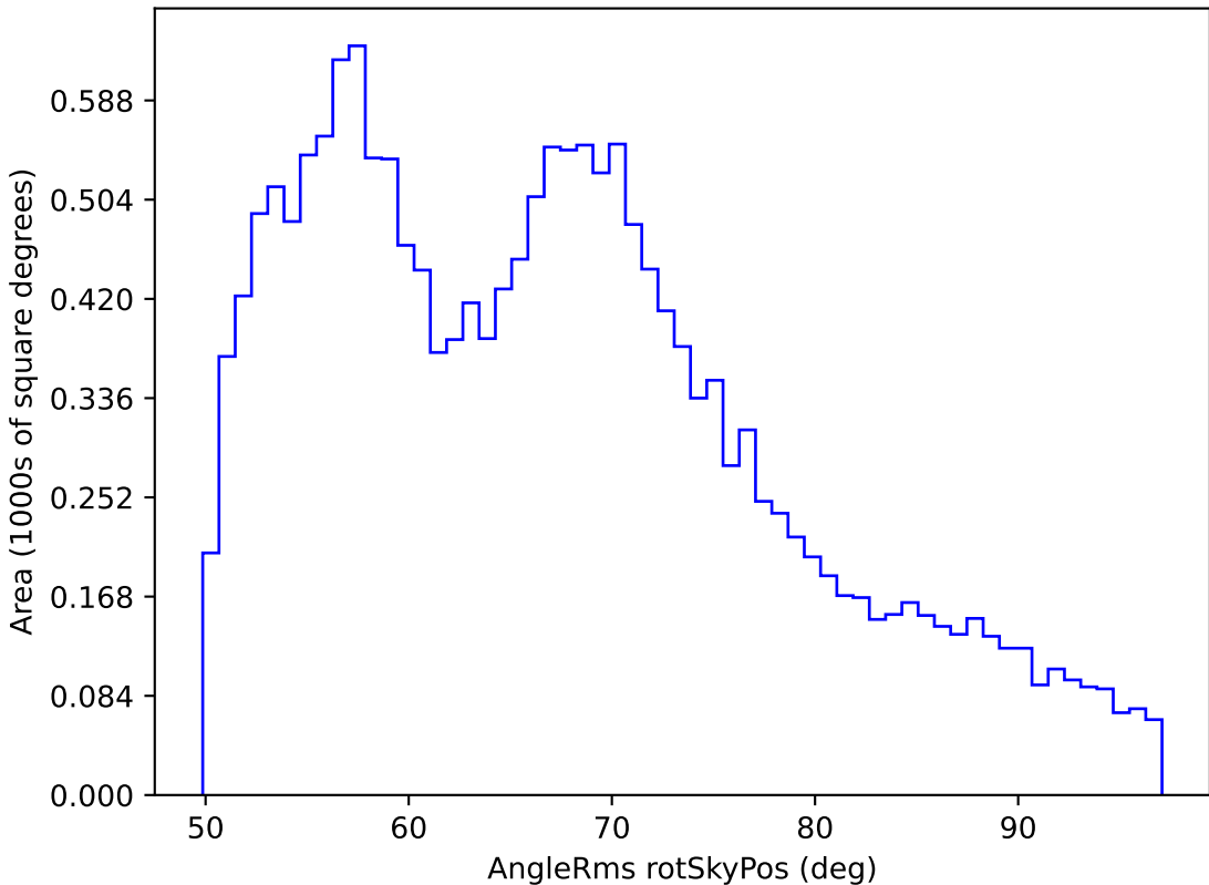
weather_cloudso6v3.4_10yrs WFD all bands: AngleRms rotSkyPos
