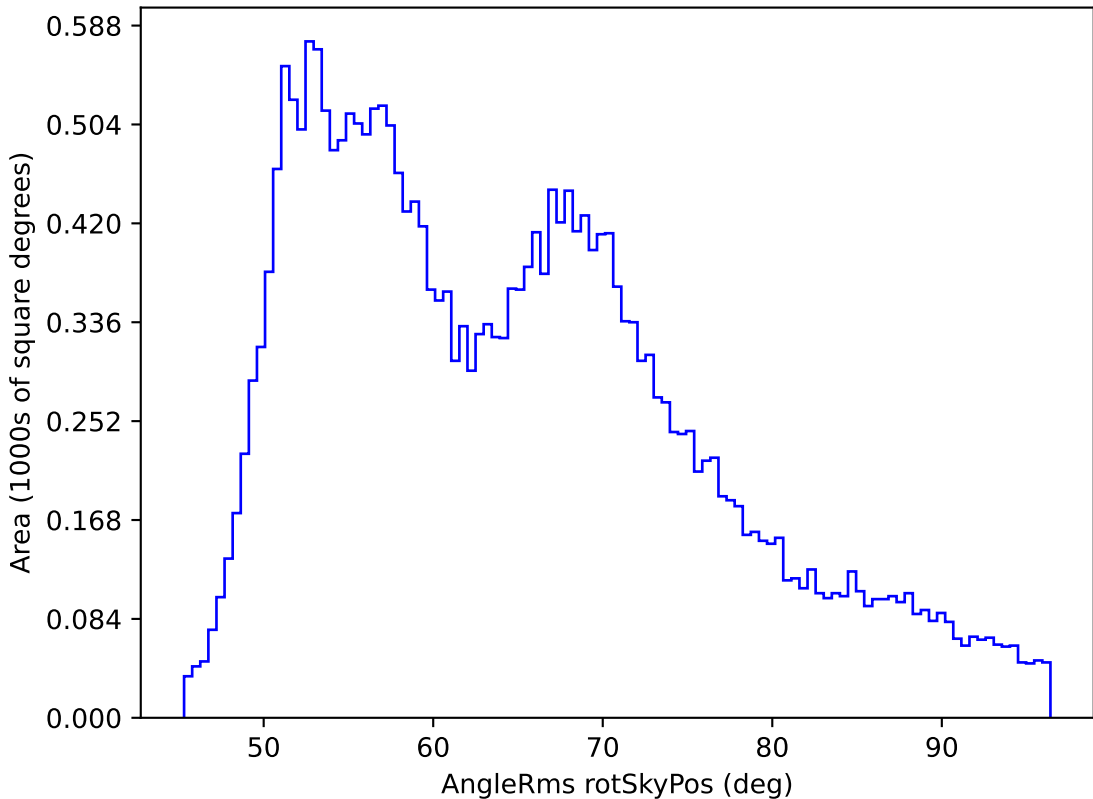
weather_cloudso6v3.4_10yrs All sky all bands: AngleRms rotSkyPos
