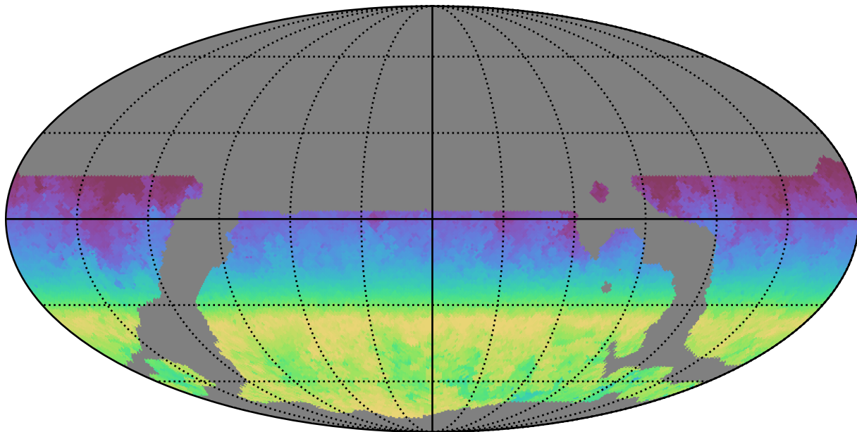
weather_cloudso6v3.4_10yrs WFD all bands: AngleRange rotSkyPos
