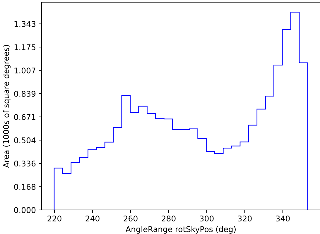
weather_cloudso6v3.4_10yrs WFD all bands: AngleRange rotSkyPos
