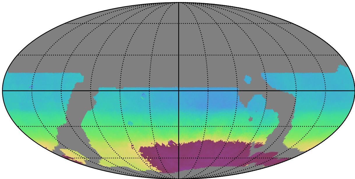
weather_cloudso6v3.4_10yrs WFD all bands: AngleMean rotSkyPos
