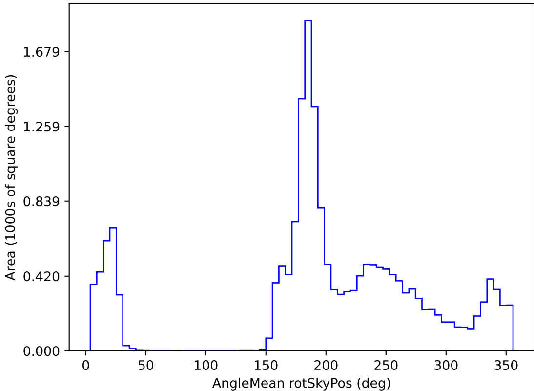
weather_cloudso6v3.4_10yrs WFD all bands: AngleMean rotSkyPos
