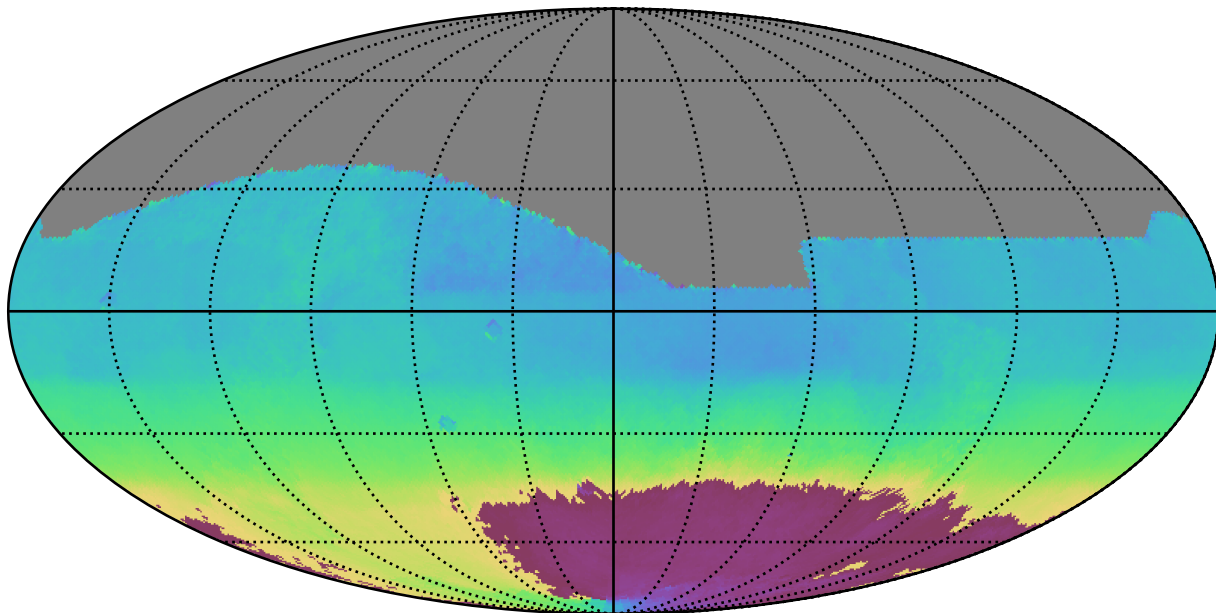
weather_cloudso6v3.4_10yrs All sky all bands: AngleMean rotSkyPos
