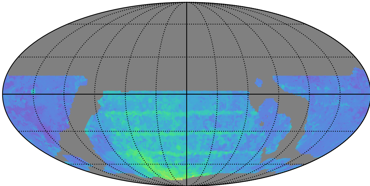
weather_cloudso6v3.4_10yrs WFD y band: 80thPercentile Season Length
