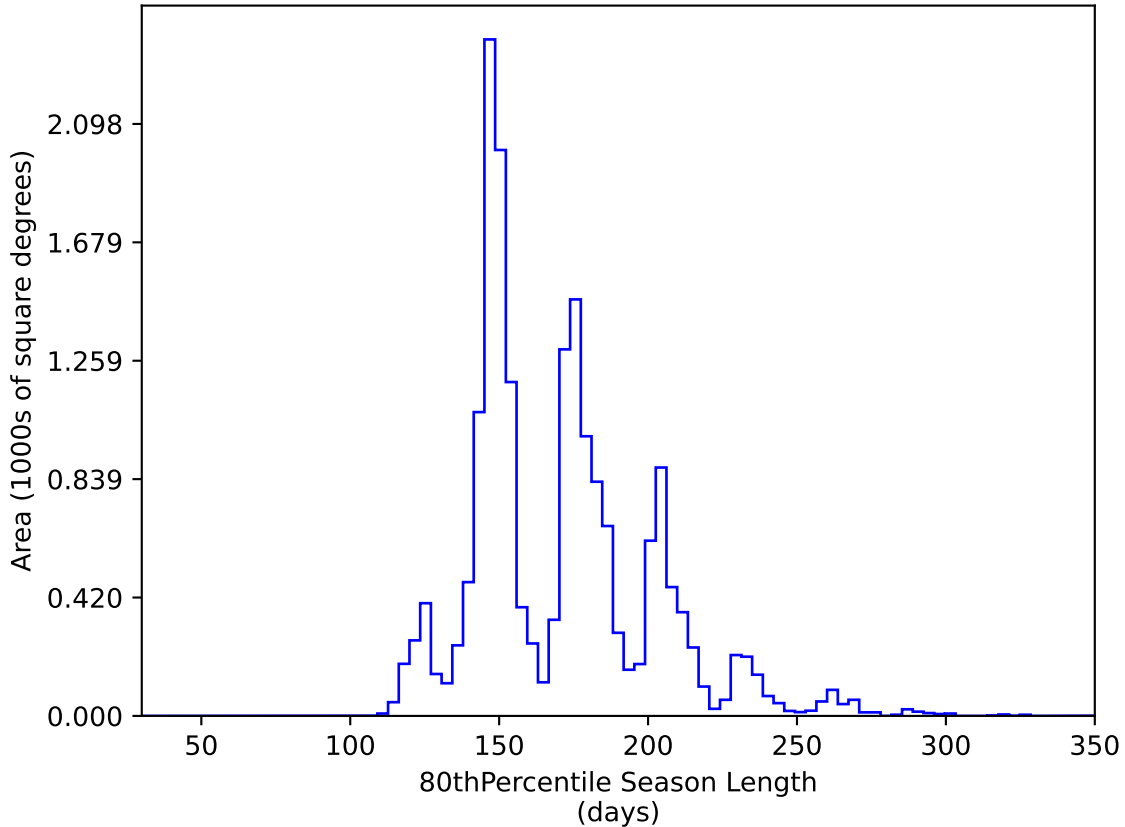
weather_cloudso6v3.4_10yrs WFD y band: 80thPercentile Season Length
