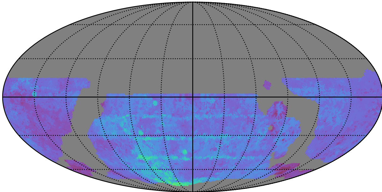
weather_cloudso6v3.4_10yrs WFD u band: 80thPercentile Season Length
