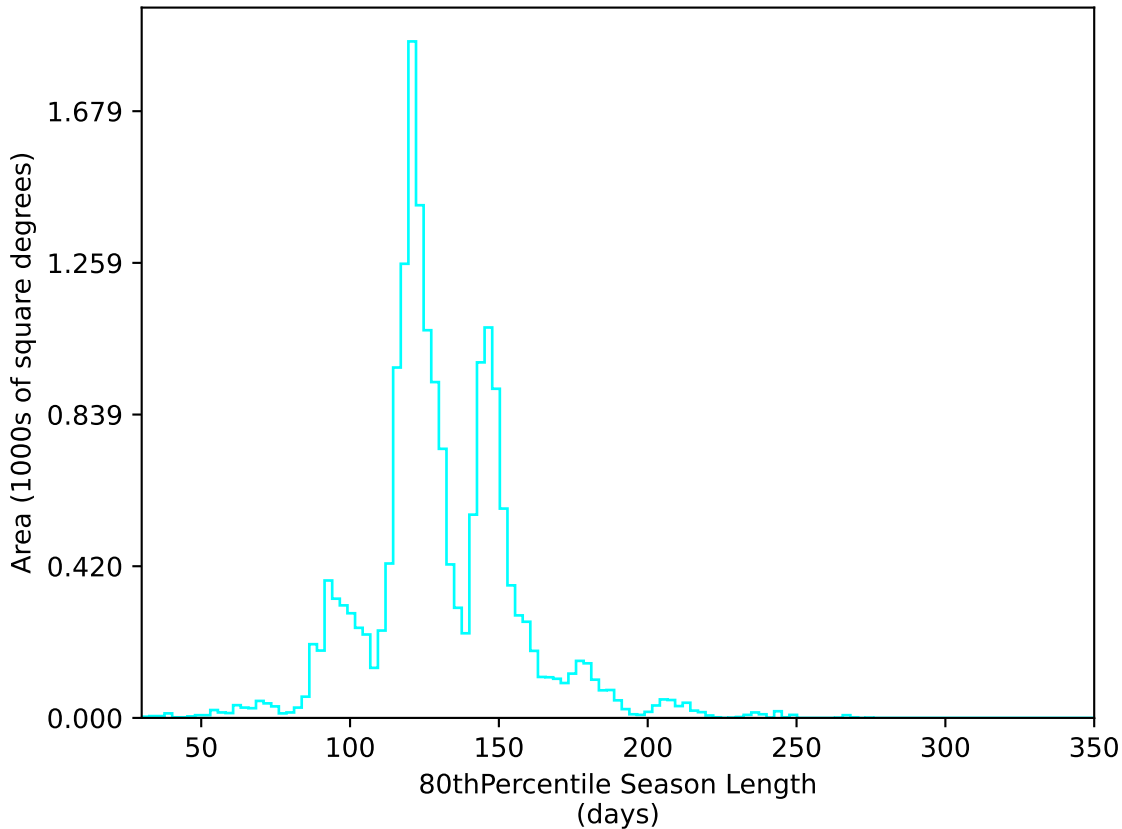
weather_cloudso6v3.4_10yrs WFD u band: 80thPercentile Season Length
