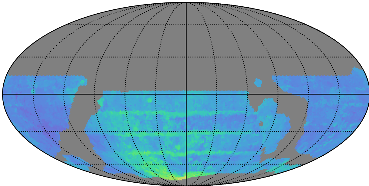
weather_cloudso6v3.4_10yrs WFD r band: 80thPercentile Season Length
