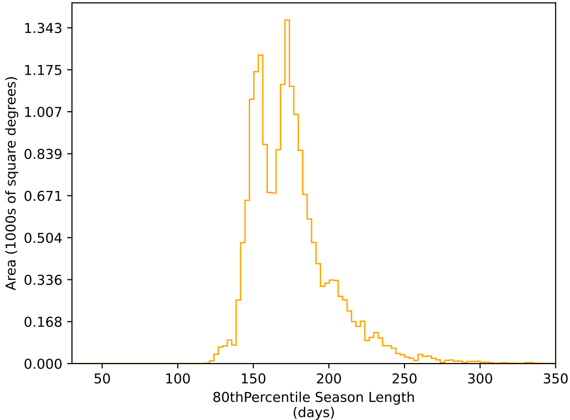
weather_cloudso6v3.4_10yrs WFD r band: 80thPercentile Season Length
