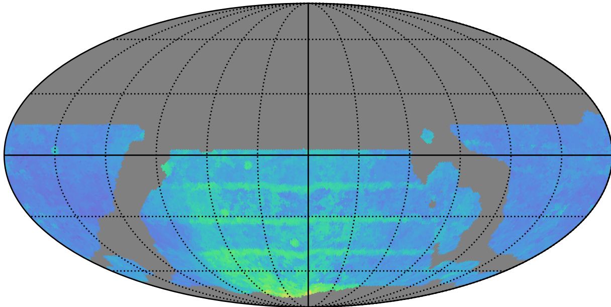
weather_cloudso6v3.4_10yrs WFD i band: 80thPercentile Season Length
